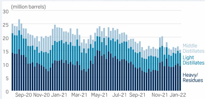
Figure 5: UAE's middle distillates stock plunge
