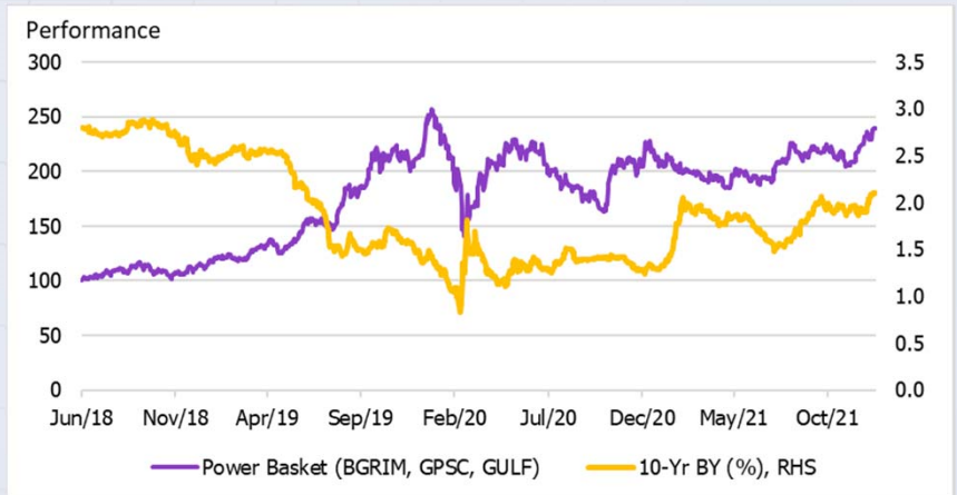
Figure 12: Utility performance vs Bond yield
