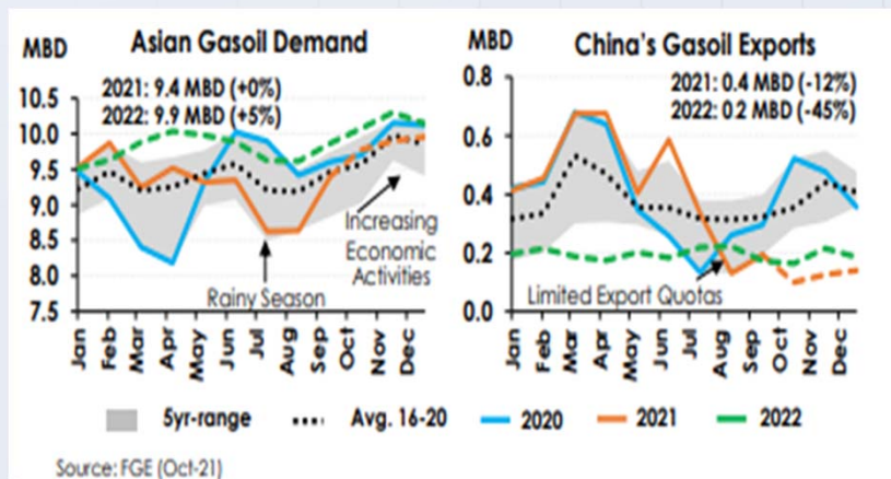
Figure 7: Asian gasoil demand to rise, China export to fall
