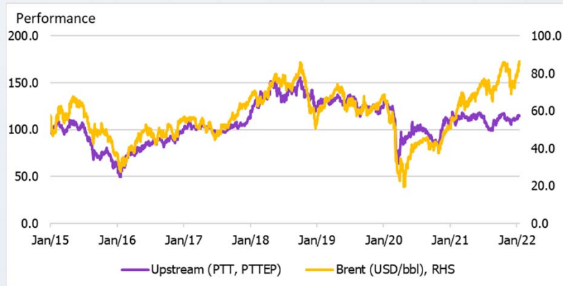
Figure 9: Divergence of the Oil and Gas vs oil prices
