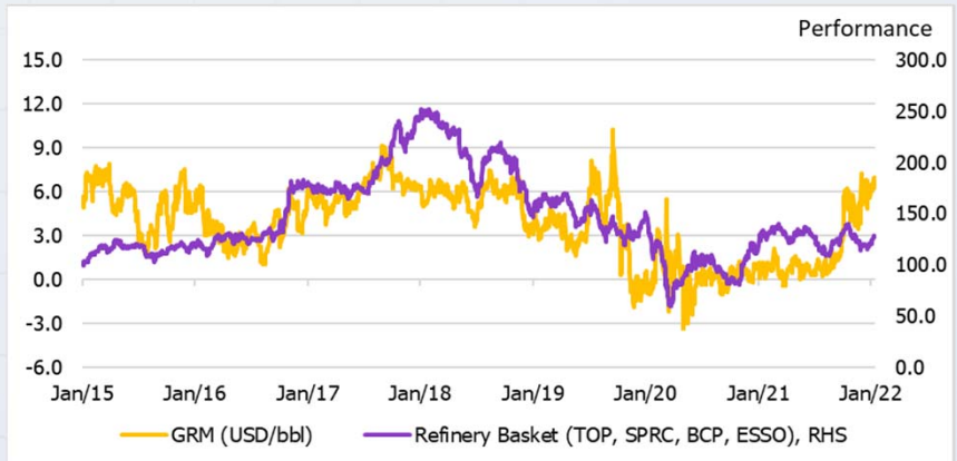
Figure 10: Refiners' shares have discounted to GRM lately
