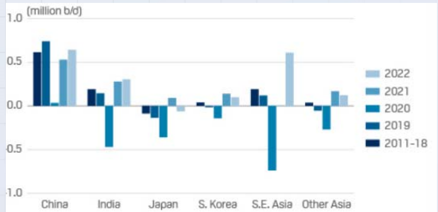
Figure 4: Asian oil demand growth on recovery path
