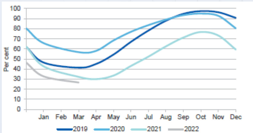
Figure 7: EU gas storage at low levels
