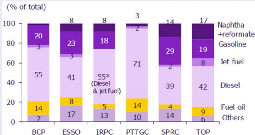
Figure 7: Thai refineries' product yields
