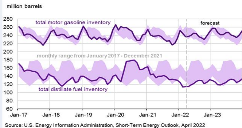
Figure 5: .S. gasoline and distillate inventories
