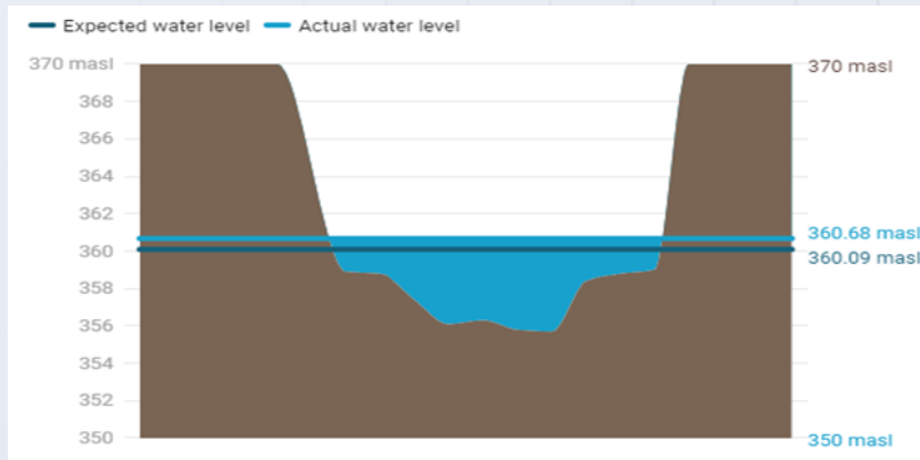
Figure 3: River levels at Chiang Saen Gauge above expected level
