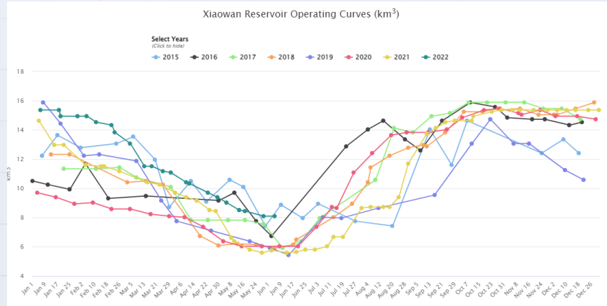
Figure 6: ... similar to Xiaowan reservoir
