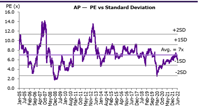
Figure 4: PER Band
