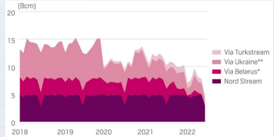
Figure 2: Gas flow from NS1 was extremely reliable in the past
