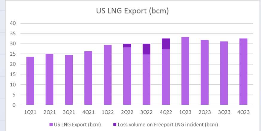
Figure 4: Without Freeport, US LNG export still grows 14% YoY
