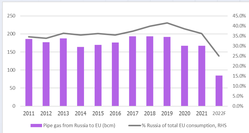
Figure 3: Gas flows to EU from Russia plunge in 2022
