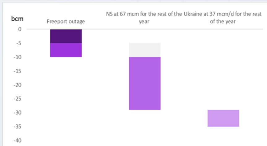
Figure 7: EU to have gas shortfall in our base case scenario
