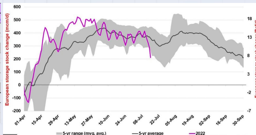
Figure 8: Eyes on the restocking rate during NS1 maintenance
