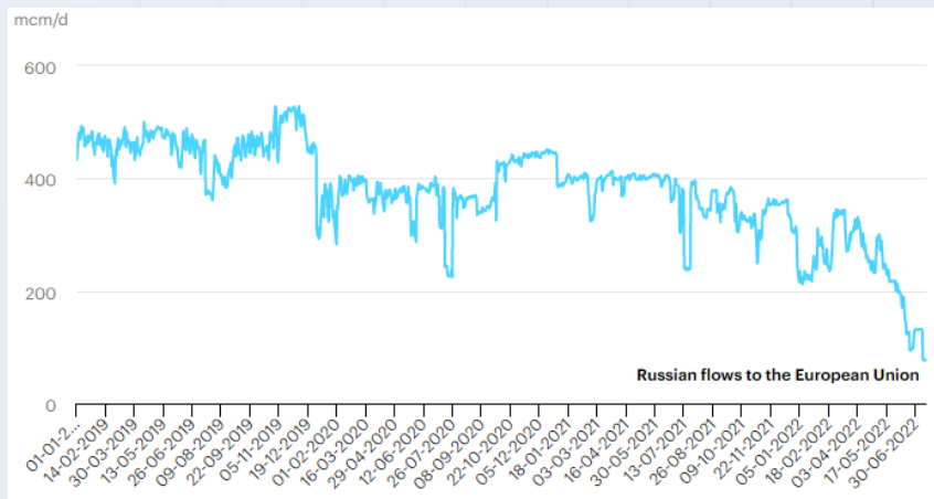
Figure 3: Russian gas flow before the resumption of NS1
