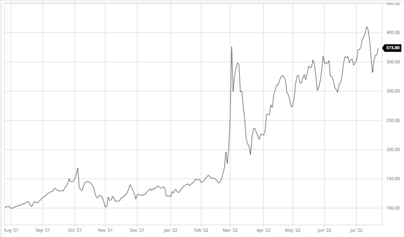
Figure 5: Newcastle coal price (USD/t)
