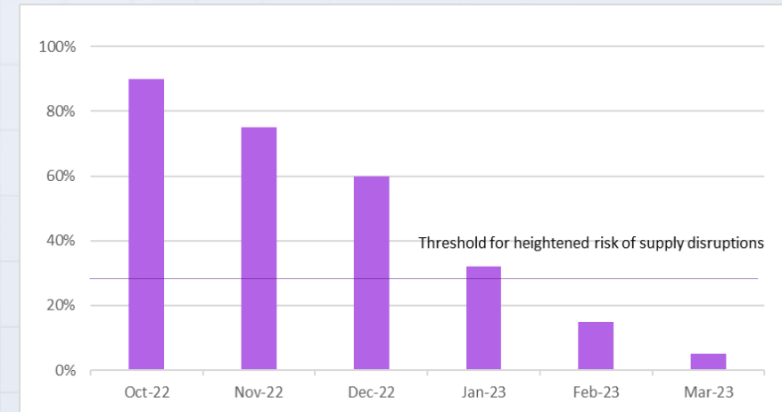
Figure 2: EU gas storage levels, if Russian supply at zero from Oct)
