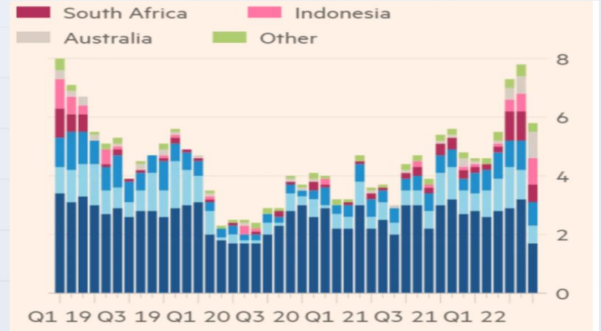
Figure 6: EU thermal coal imports in mt
