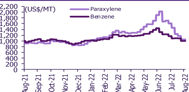
Aromatics prices
