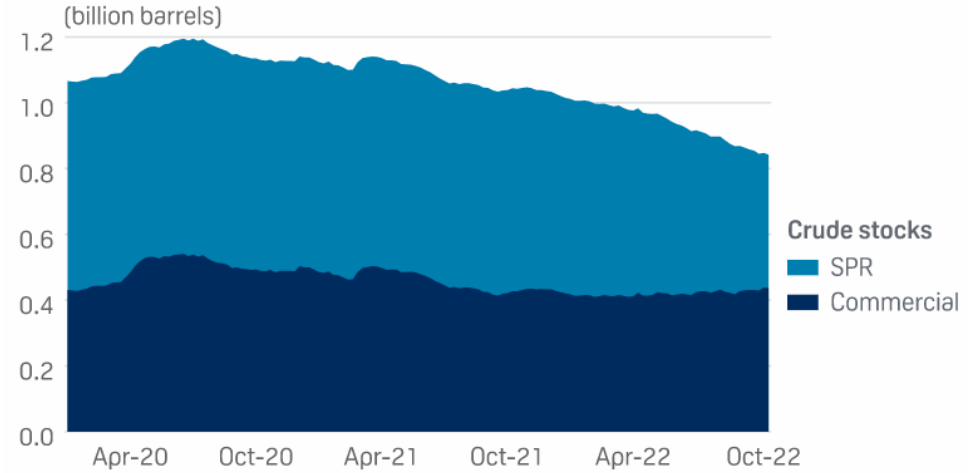
Figure 4: US commercial crude inventories
