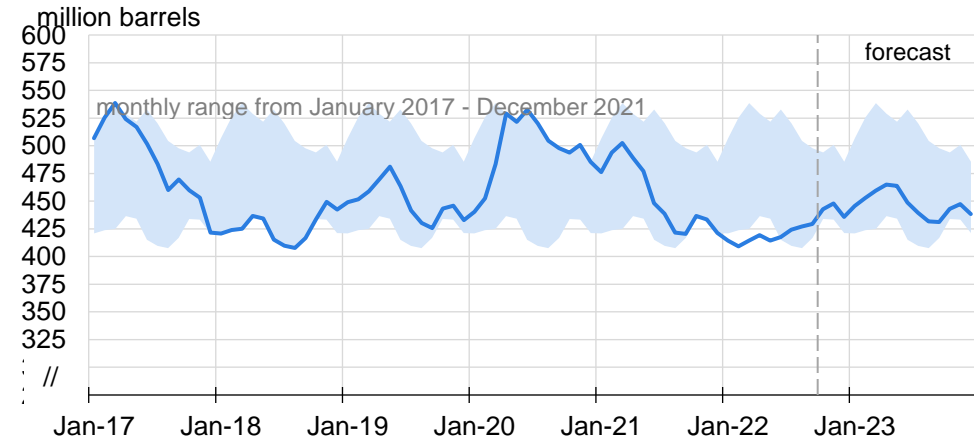
Figure 4: US commercial crude inventories
