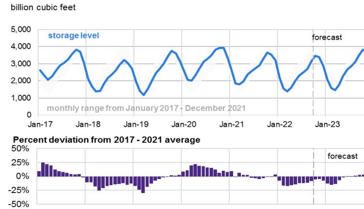
Figure 8: US natural gas in storage
