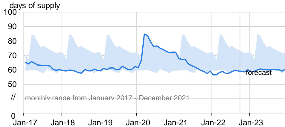
Figure 3: OECD commercial inventory below 5-year rage
