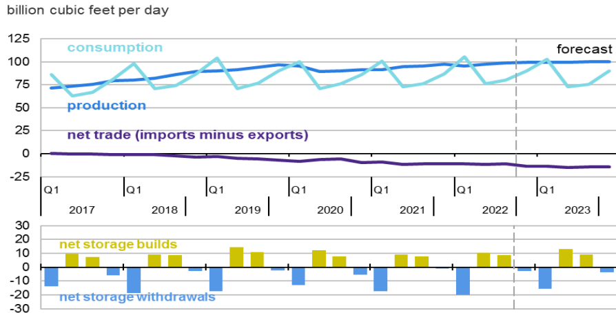
Figure 7: US natural gas production, consumption and net imports
