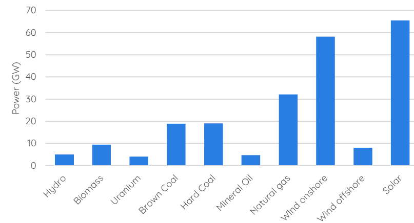
Figure 4: Net Installed Electricity Generation Capacity in Germany in 2022
