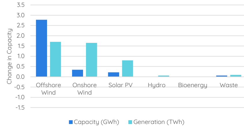
Figure 4: Net Installed Electricity Generation Capacity in Germany in 2022
