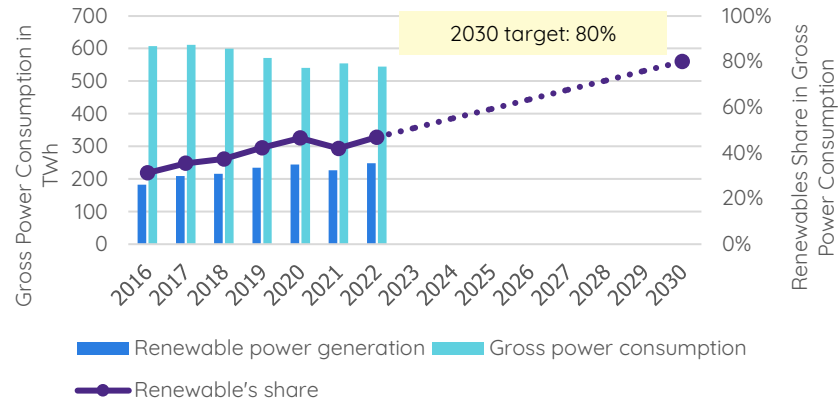
Figure 5: Renewable's Shares in Germany Power Consumption
