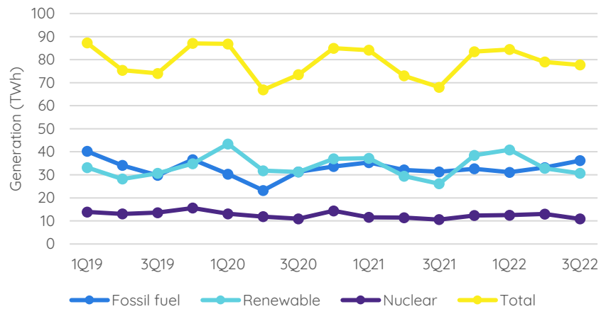
Figure 3: UK Electricity Generated, by Fuel Type
