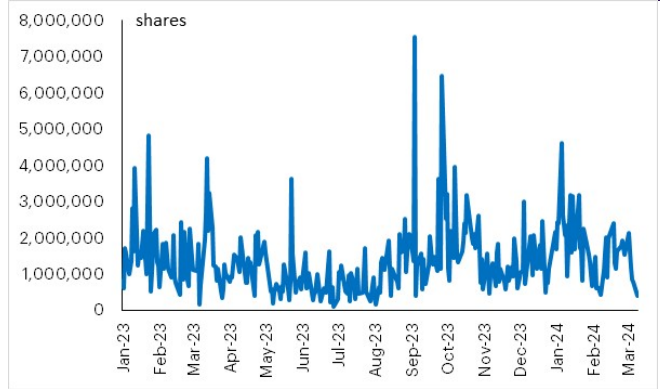
Figure 4: Daily SCGP & SCGP-R Short Sales
