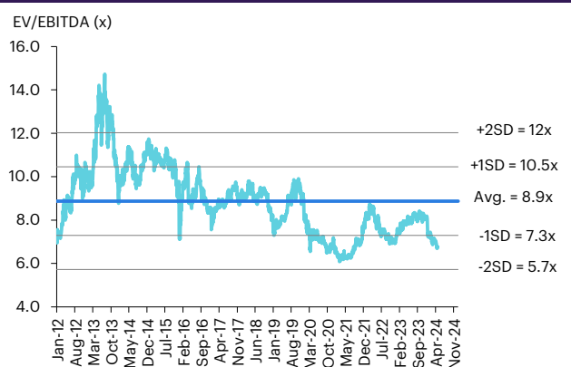
Figure 9: EV/EBITDA Band
