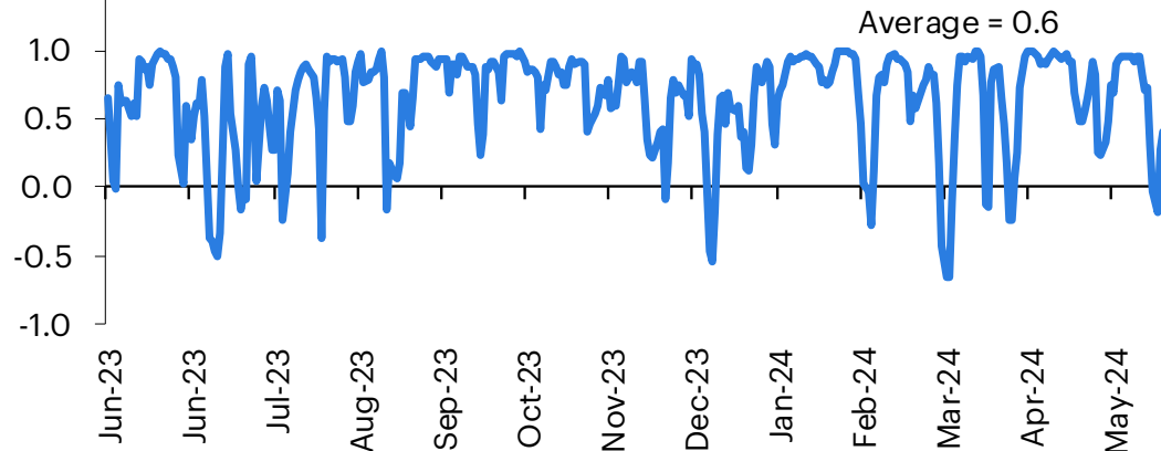
SOL correlation to BTC
