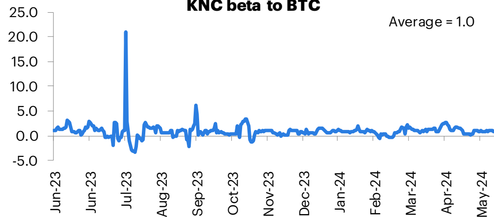
KNC beta to BTC
