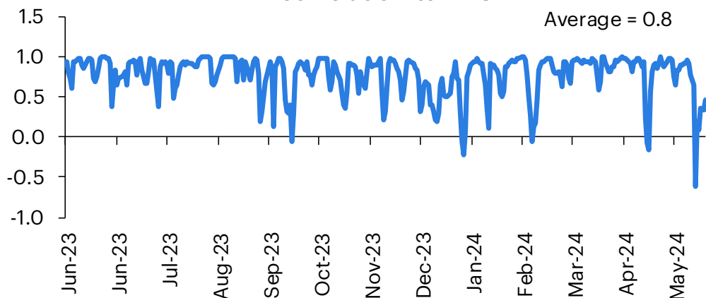
ETH correlation to BTC
