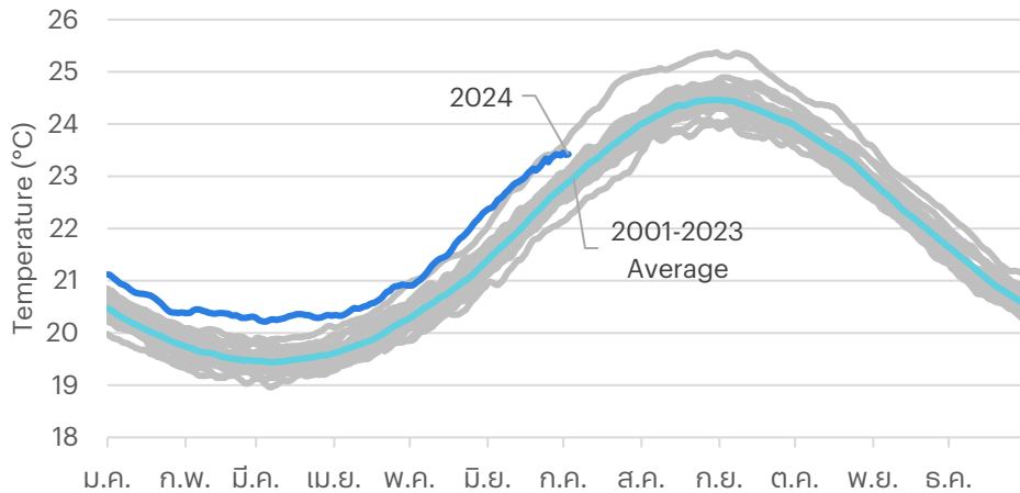
Figure 3: High Sea Surface Temperature Driving Strong Monsoon Season
