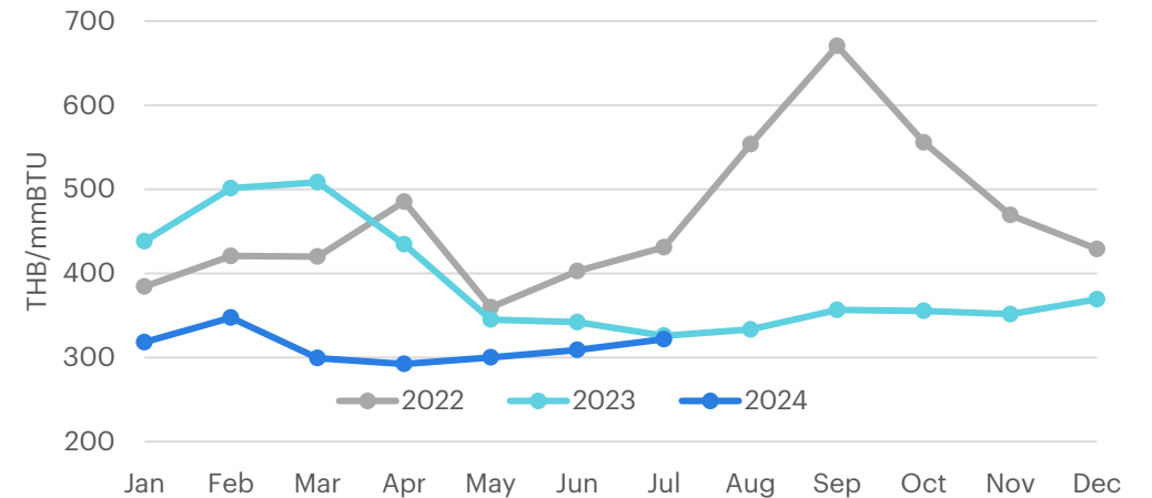
Figure 8: Thailand's Energy Pool Price On an Upward Trend
