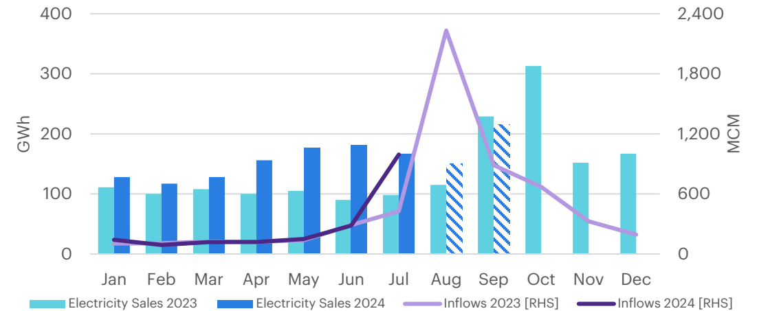
Figure 4: NN2 Water Inflow Start to Rise YoY in July
